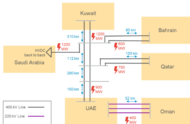
Figure 19: Schematic presentation of the GCC interconnection grid. 101
