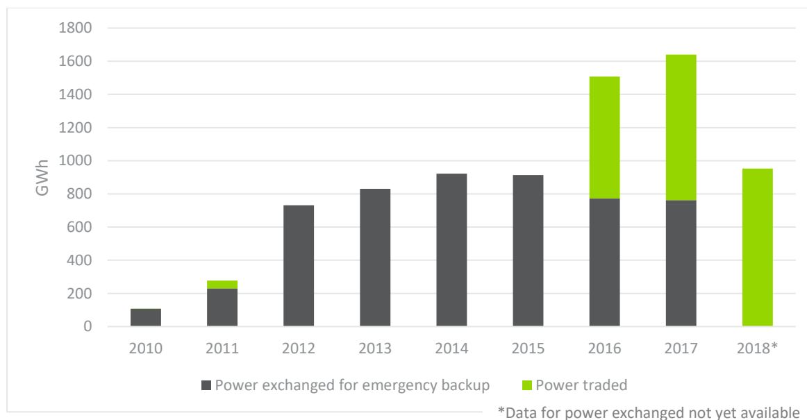
Figure 21: Volume of power exchanged & traded on the GCC interconnection grid. 121
