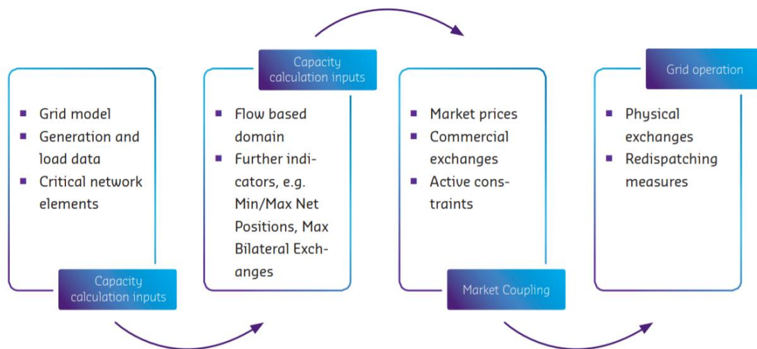
Figure 3: Overview over flow-based capacity calculation and allocation. 45
