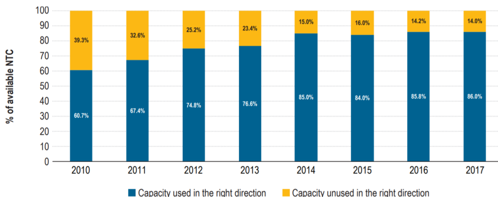
Figure 5: Utilization of interconnections in day-ahead market timeframe in times of significant price differentials (>1 Euro/MWh) on 37 European electricity borders. 58
